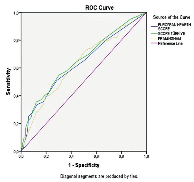
Figure 2: ROC curve analysis. ROC: Receiver operating characteristic
